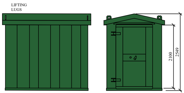
APEX ROOF PAINTED PROFILE STEEL OUTER FINISH
