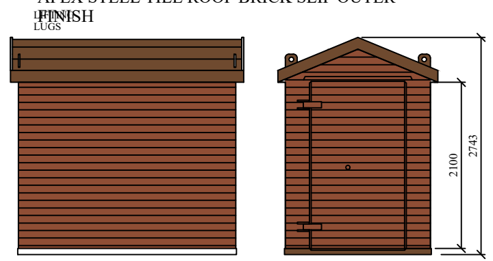
TILE EFFECT ROOF TIMBER CLAD OUTER FINISH
