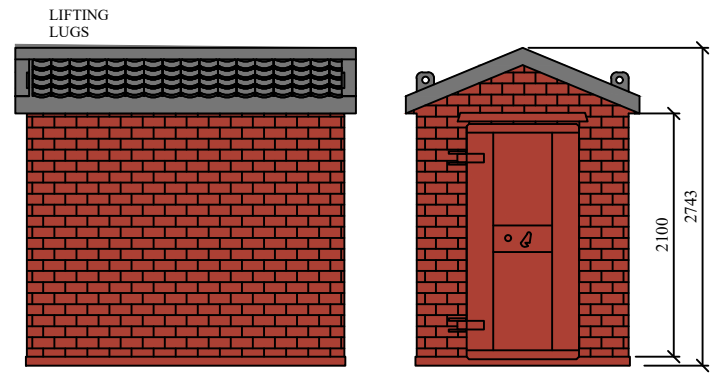
APEX STEEL TILE ROOF BRICK SLIP OUTER FINISH
